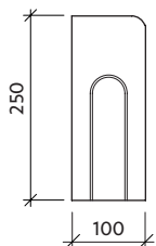
bokorys T 8
