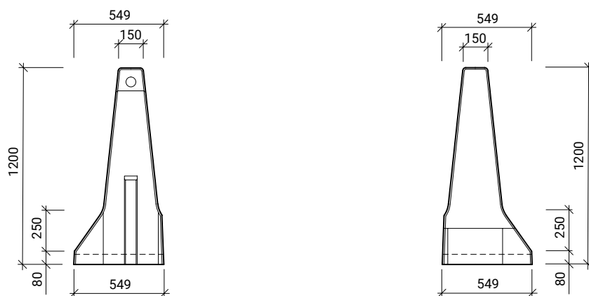
Bokorys
